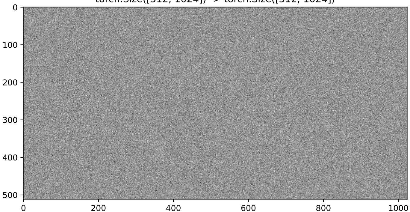
Distribution of the first tensor
